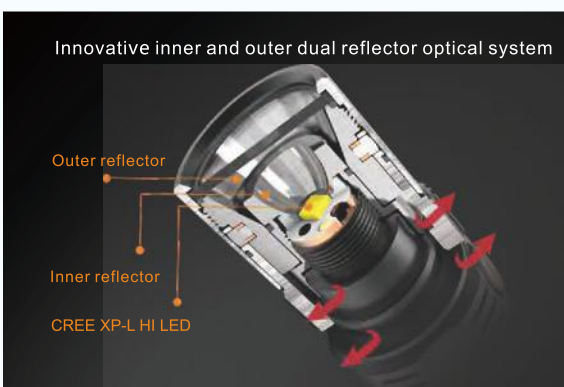
Dual reflector optical system
