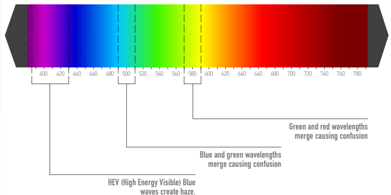
LIGHT SPECTRUM SEEN WITH THE NAKED EYE
